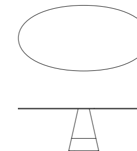
ART. TFRO180 L/W 180 H 74 P/D 110 W 70,9" H 29,1" D 43,3"
