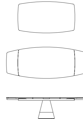
ART. TFR200A L/W 200/240/280 H 74 P/D 110 W 78,7"/94,5"/110,2" H 29,1" D 43,3"
