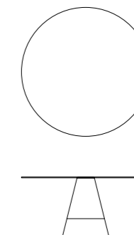
ART. TFR120 Ø 120 H 74 Ø 47,2" H 29,1"
